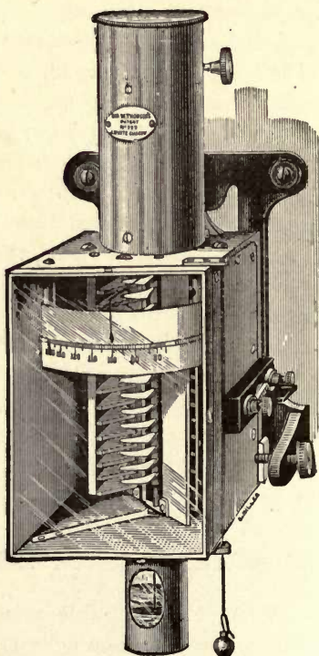
Fig. 172.—Kelvin Multicellular Voltmeter (Engine-Room vertical pattern)
